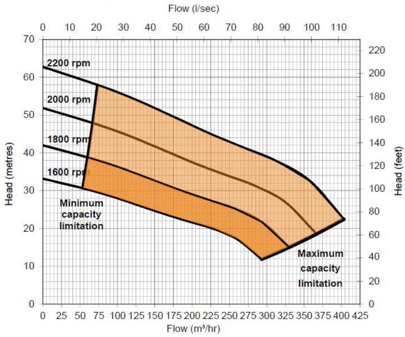
Perkins 404D22T FC (33.5 kW@ 1800 rpm)
